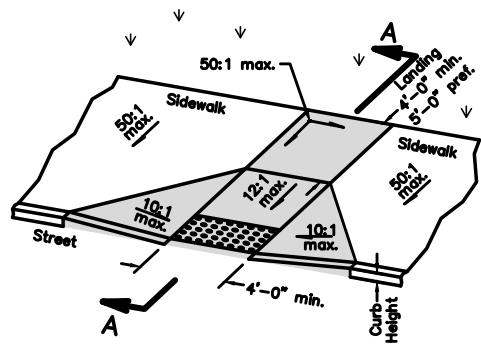
Type A1 (Perpendicular with flared sides)
