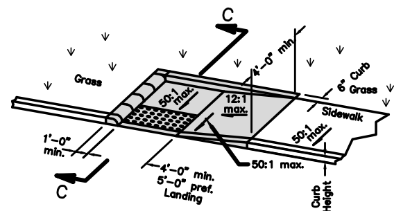
Type B1 (Single sided Parallel)
