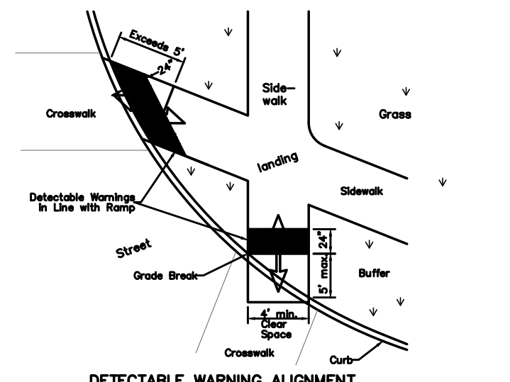
DETECTABLE WARNING ALIGNMENT
