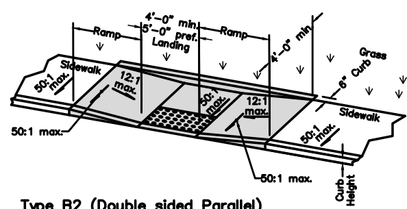
Type B2 (Double sided Parallel)
