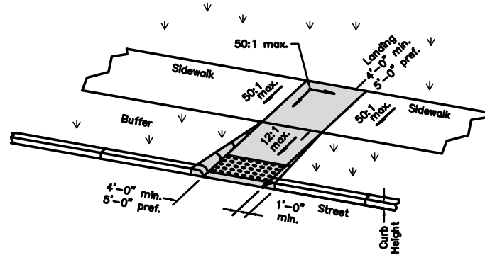
Type A2 (Perpendicular with returned curb)
