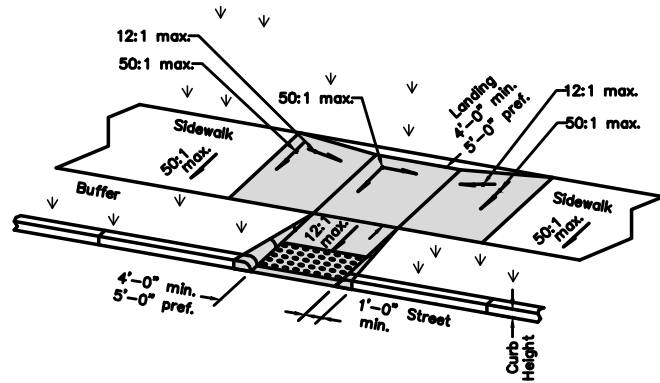
Type C2 (Combined with returned curb)
