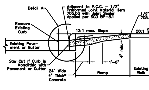
SECTION A-A EXISTING WALK DETAIL
