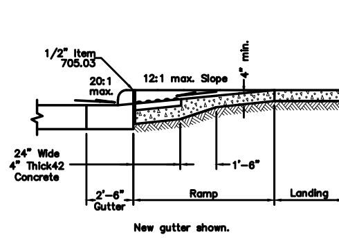
SECTION A-A NORMAL DETAIL
